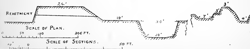
SECTION OF MAIN WORK.
